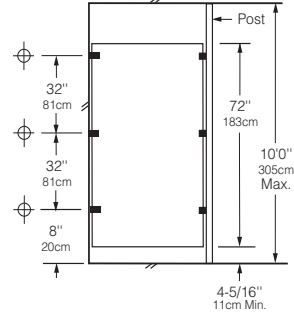
2093 Series Post-to-Ceiling Screen
