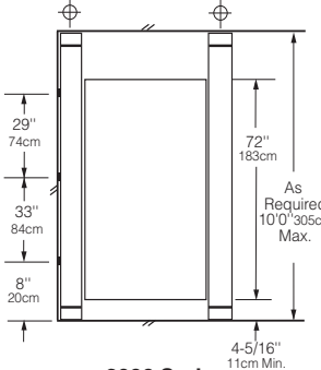
2096 Series Floor-to-Ceiling Anchored
