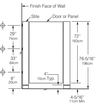
2090 Series Floor-Anchored
