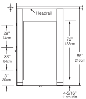
2092 Series Overhead-Braced
